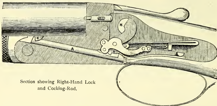
Mechanism of Scott's Hammerless Gun.
